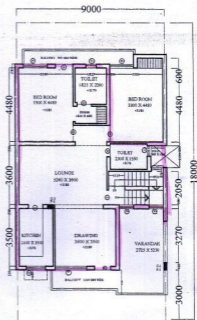
FIRST FLOOR PLAN (FUTURE)
