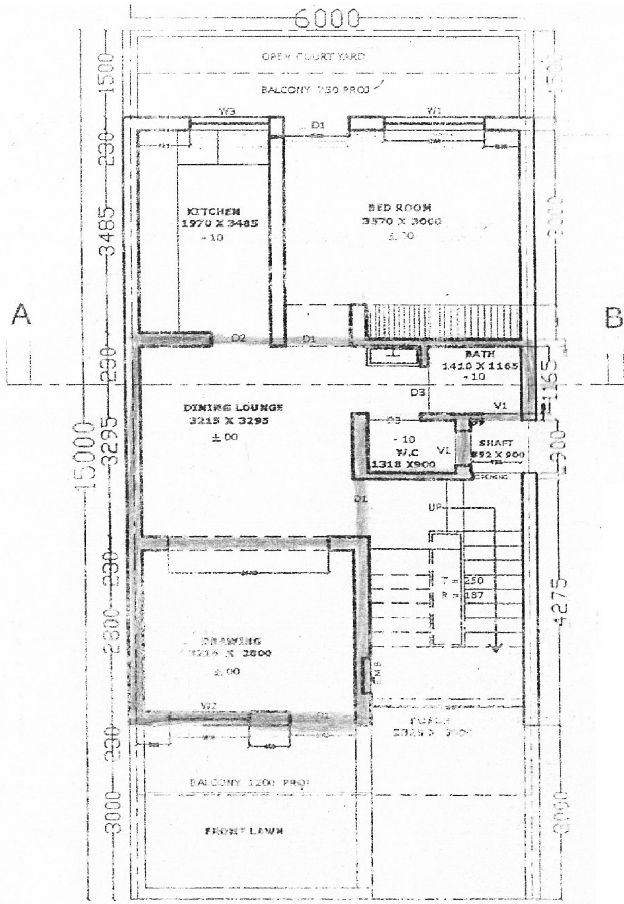
GROUND FLOOR PLAN LIG (06.00 x 15.00 mtr.)
