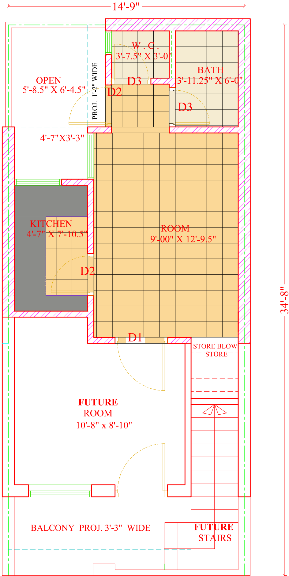
EWS House (Plinth Area - 238.95 Sqft)
