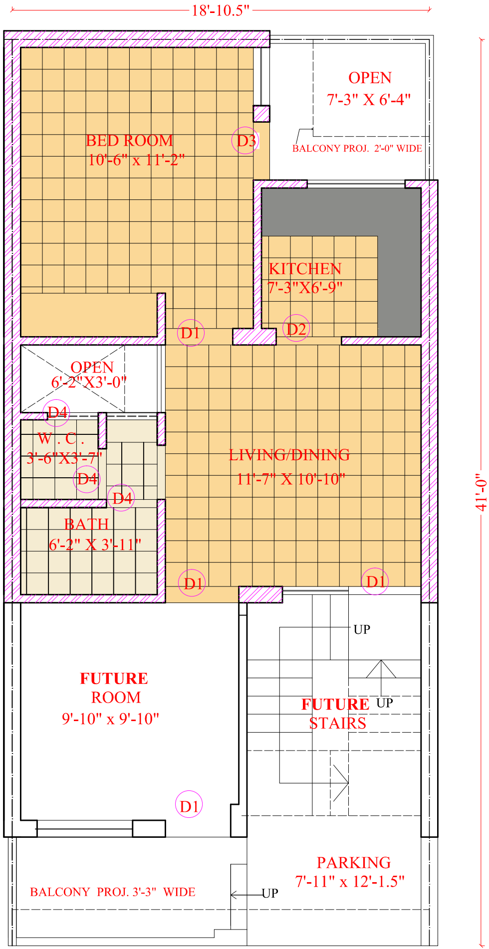
LIG House (Plinth Area - 414.70 Sqft)
