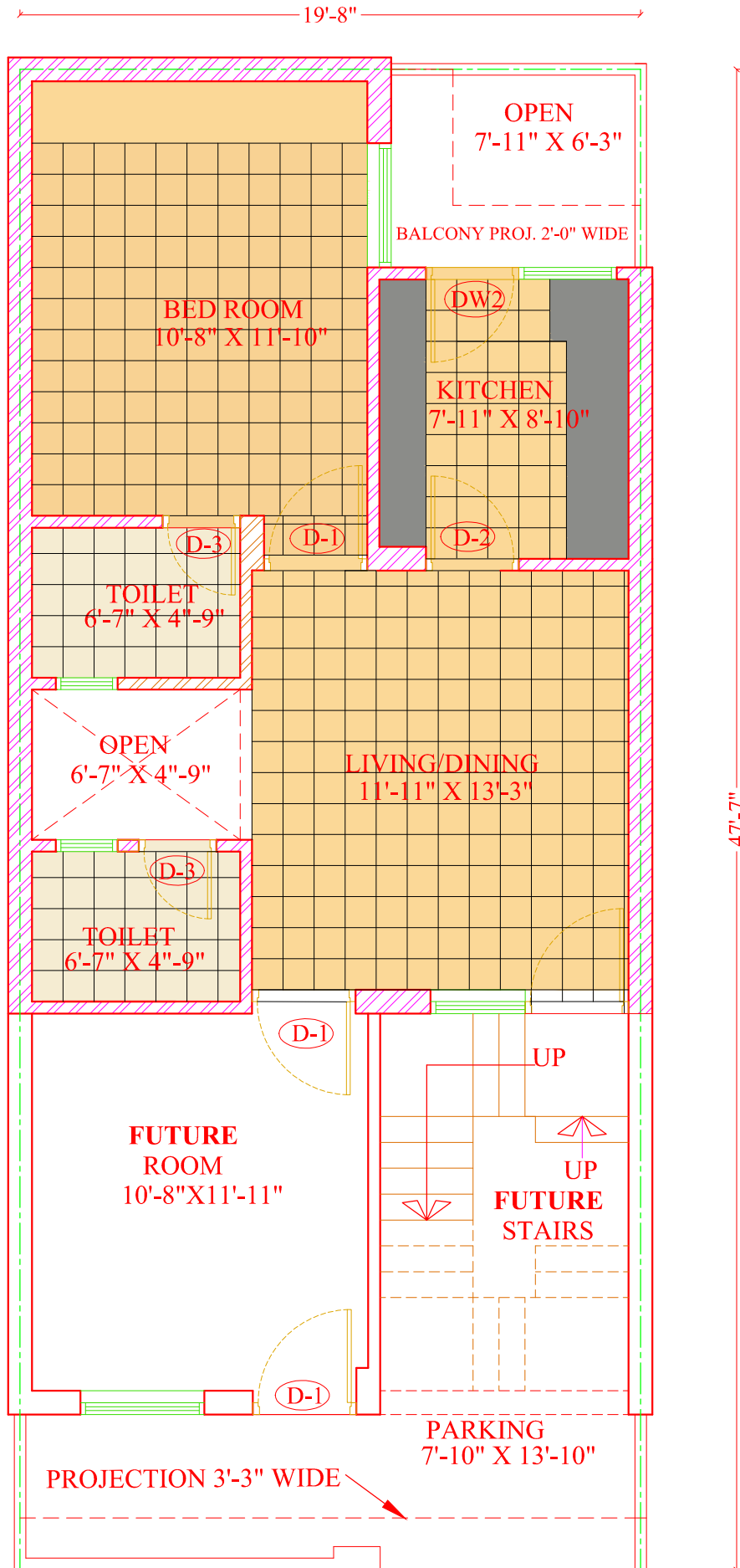
MIG-A House (Plinth Area = 506.25 Sqft)
